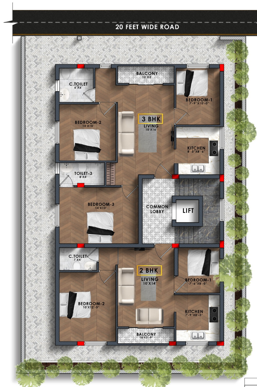
TYPICAL FLOOR PLAN(3 FLOORS)
